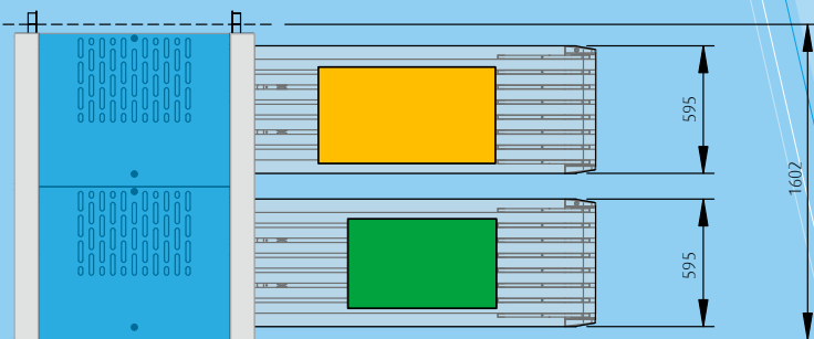
Top view - two single stackers working as twin stacker. All measures are stated in mm.
