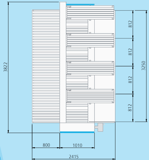
Typical layout - all measures are stated in mm
