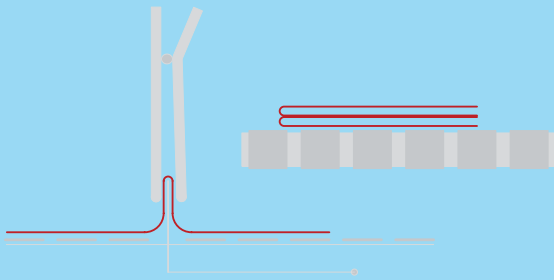
Crossfolding by the fold & stack system
